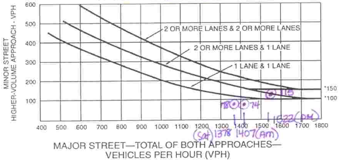
Figure 4C-3. Warrant 3, Peak Hour Camino Capistrano @ Forster Rd 2015 Cumulative Conditions
